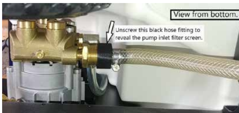
Figure 10 – Location of pump filter screen.
