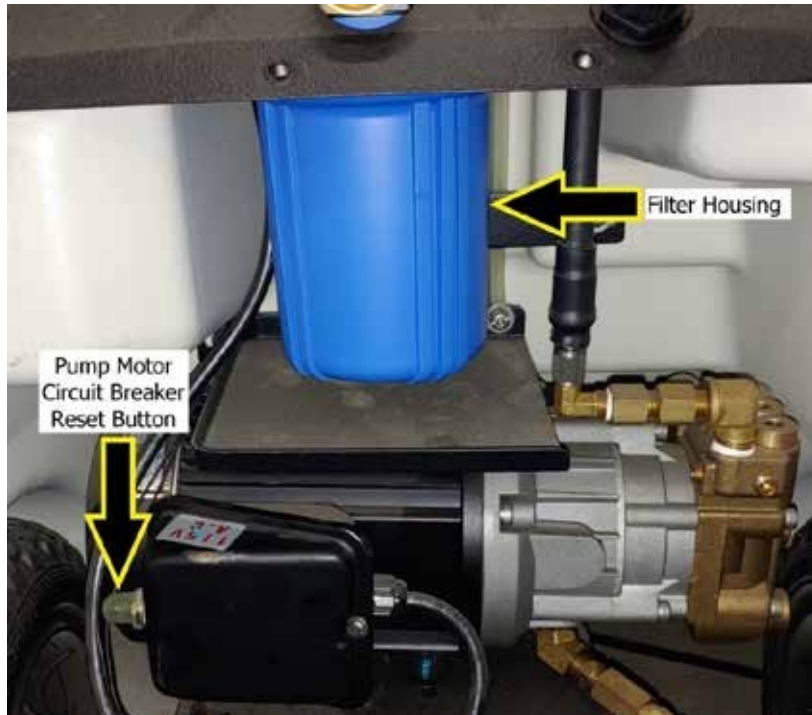
Figure 9 – Location of filter housing and circuit breaker reset button.
